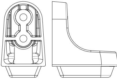
Door bump stop Profile Art. No. 373706
