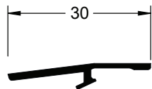
Finishing trim Profile Art. No. 362276
