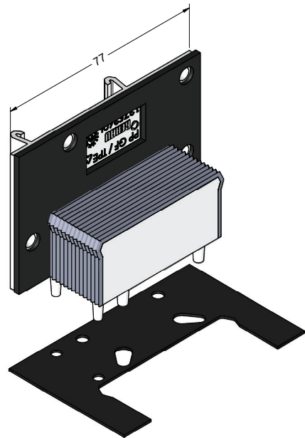
Mechanical joint block Left hand Art. No. 375460 Right hand Art. No. 375360
