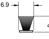
Brushpile 6.9 x 8mm Profile Art. No. 371038
