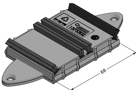
Anti-lift block Profile Art. No. 375302
