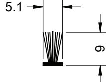
Brushpile 5.1 x 9mm Profile Art. No. 357855
