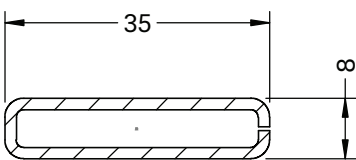
Reinforcement 35 x 8 x 1.5mm Art. No. 357864
