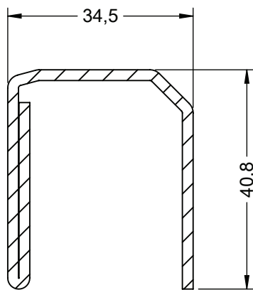
Reinforcement 34.5 x 40.8 x 2mm Art. No. 357832
