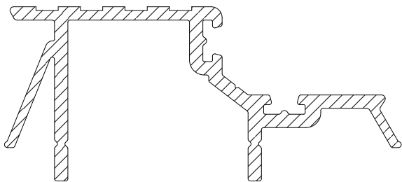
Tread plate Profile Art. No. 357843
