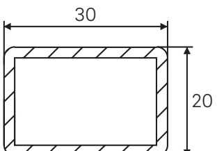
Reinforcement 30 x 20 x 1mm Art. No. 324971 Reinforcement 30 x 20 x 2mm Art. No. 255924
