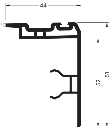
Interlock White Profile Art. No. 575506 Laminated Profile Art. No 595606
