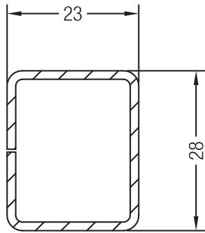
Reinforcement 23 x 28 x 1.5mm Art. No. 357540
