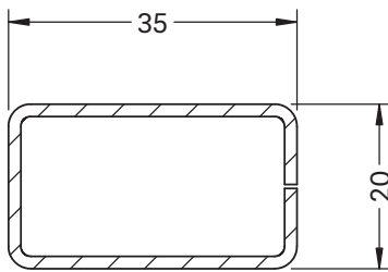
Reinforcement 35 x 20 x 1.5mm Art. No. 357836
