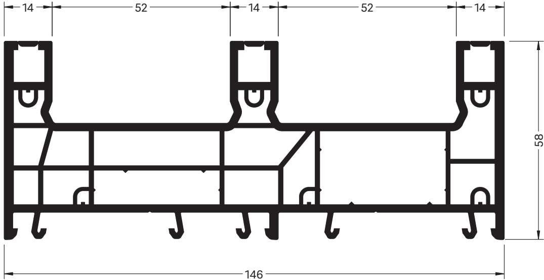
Triple track frame White Profile Art. No. 575603 Laminated Profile Art. No 595803 Reinforcement 35 x 20 & Reinforcement 35 x 8
