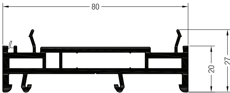
20mm frame extension White Profile Art. No. 538025 Laminated Profile Art. No 568025 Reinforcement 35 x 6
