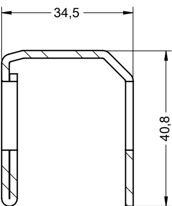
Reinforcement 34.5 x 40.8 x 2mm (Pre-routed) Art. No. 361488
