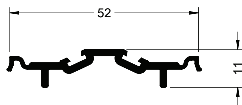
Thermal profile incl. drainage holes Profile Art. No. 575622 Thermal profile - no drainage holes Profile Art. No. 575722
