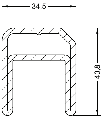
Reinforcement 34.5 x 40.8 x 2.5mm Art. No. 357833
