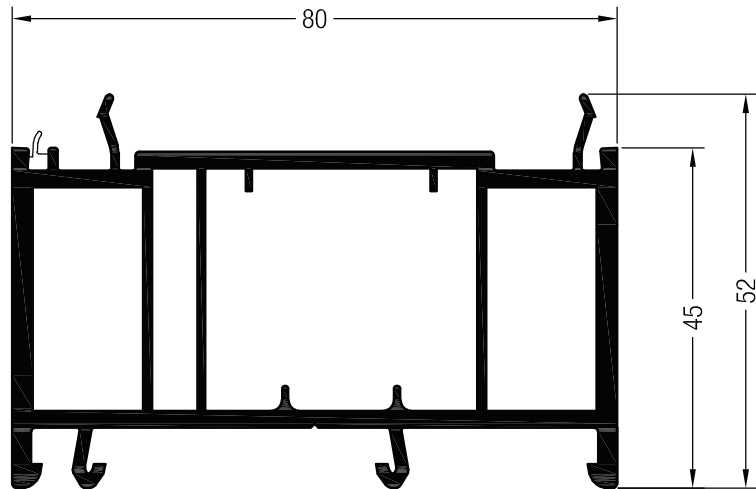
45mm frame extension White Profile Art. No. 538045 Laminated Profile Art. No 568045 Reinforcement 23 x 28
