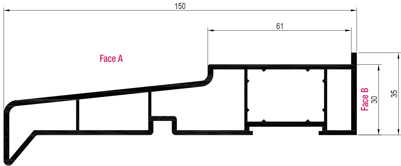
150mm sill White Profile Art. No. 246330 Laminated Profile Art. No 246360 Reinforcement 30 x 20
