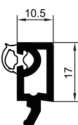
28mm Glazing bead White Art. No. 559605 Laminated Art. No. 589605
