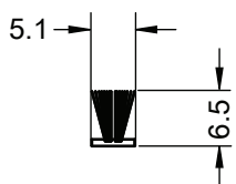
Brushpile 5.1 x 6.5mm Profile Art. No. 334728
