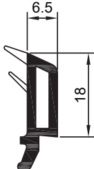
32mm Glazing bead White Art. No. 560580 Laminated Art. No. 594330
