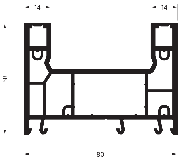
Door frame White Profile Art. No. 575602 Laminated Profile Art. No 595802 Reinforcement 35 x 20
