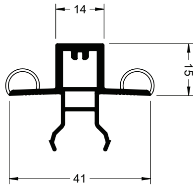
3/4 pane seal Profile Art. No. 575507
