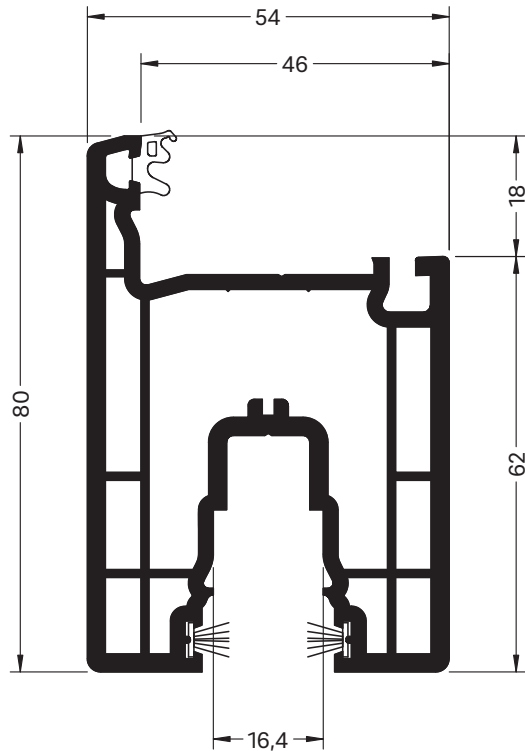
Door sash White Profile Art. No. 575305 Laminated Profile Art. No 595405 Reinforcement 34.5 x 40.8
