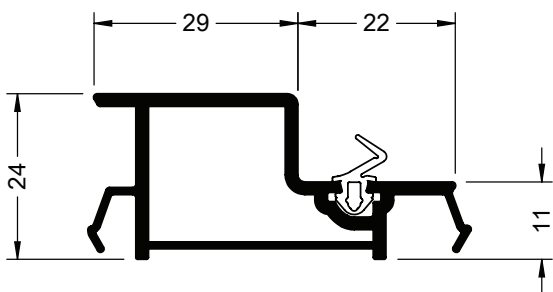
Cover profile White Profile Art. No. 575626 Laminated Profile Art. No 595726
