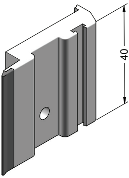
Interlock seal end cap Profile Art. No. 375308
