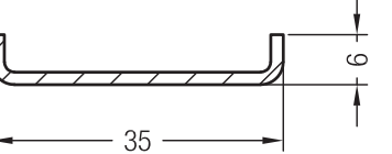
Reinforcement 35 x 6 x 1.5mm Art. No. 361002
